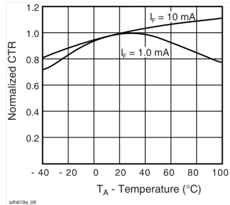
Fig. 8 - Normalized CTR vs. Temperature
