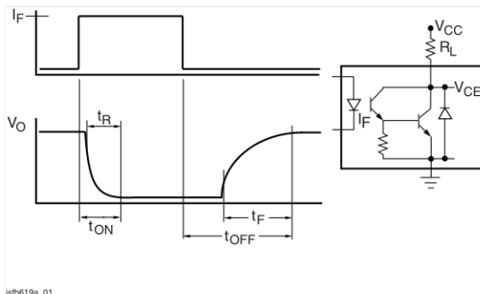
Fig. 1 - Switching Waveform and Switching Schematic
