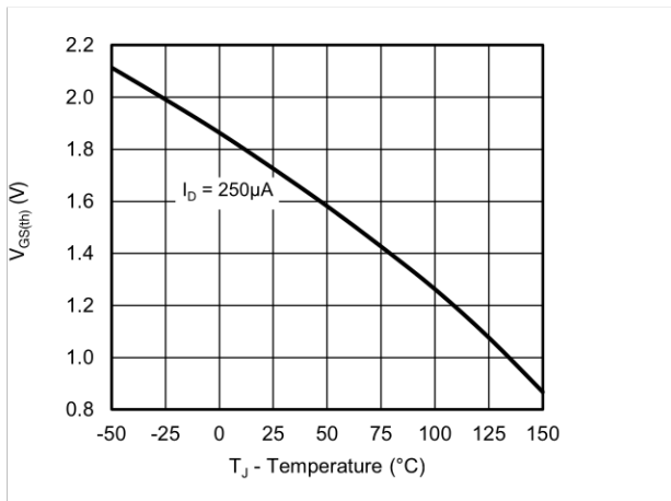
Threshold Voltage
