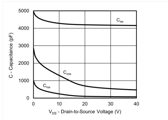
Capacitance
