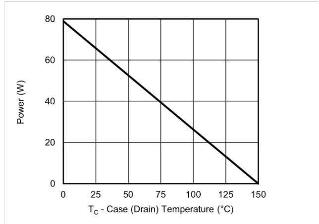
Power, Junction-to-Case
