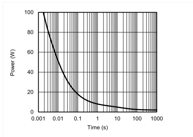
Single Pulse Power, Junction-to-Ambient
