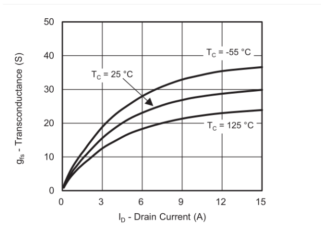
Transconductance
