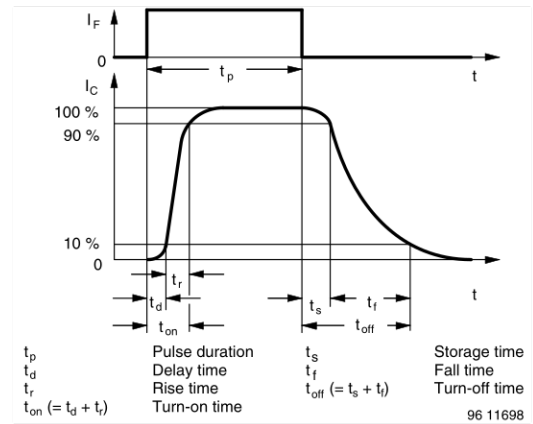
Fig. 5 - Switching Times
