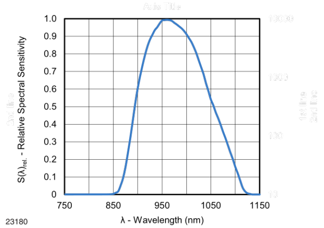
Fig. 10 - Relative Spectral Sensitivity vs. Wavelength
