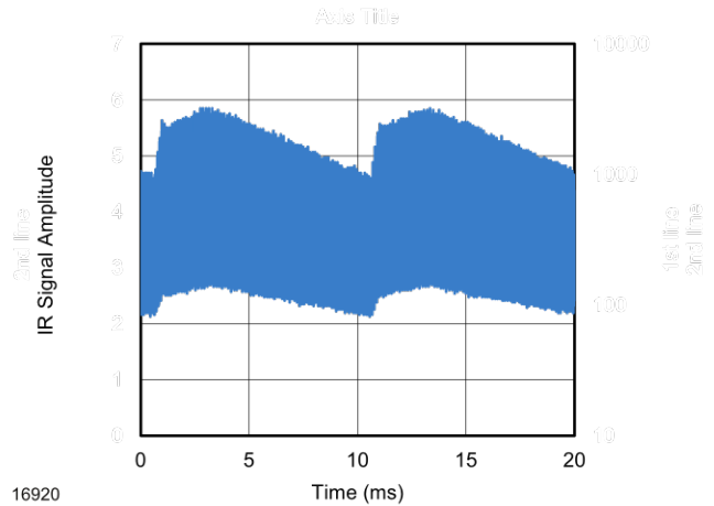
Fig. 13 - IR Disturbance from Fluorescent Lamp With Low Modulation
