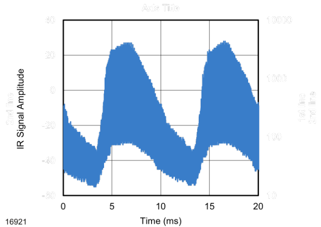
Fig. 14 - IR Disturbance from Fluorescent Lamp With High Modulation
