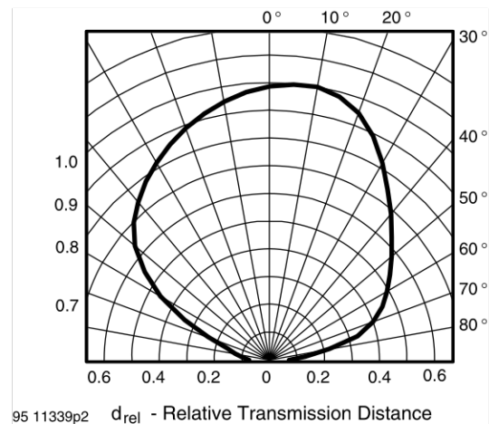
Fig. 13 - Vertical Directivity
