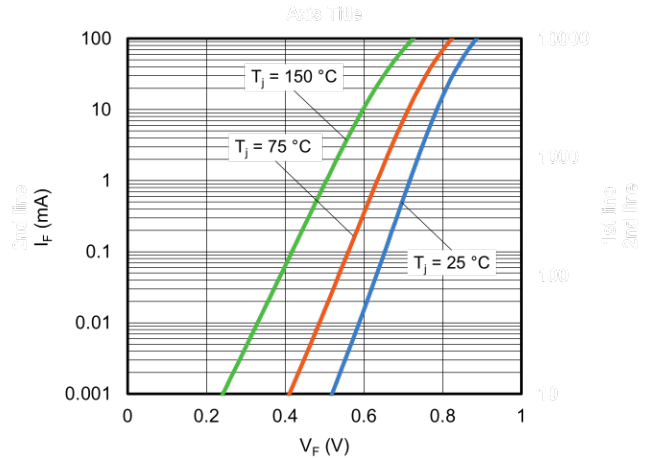
Fig. 5 - Typical Forward Current I_F vs. Forward Voltage V_F
