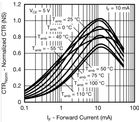
Fig. 11 - Normalized CTR (NS) vs. Forward Current
