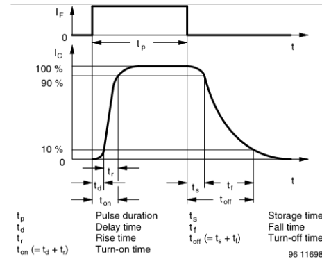
Fig. 4 - Switching Times
