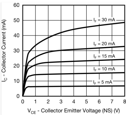
Fig. 6 - Collector Current vs. Collector Emitter Voltage (NS)
