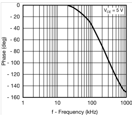
Fig. 13 - CTR Frequency vs. Phase Angle
