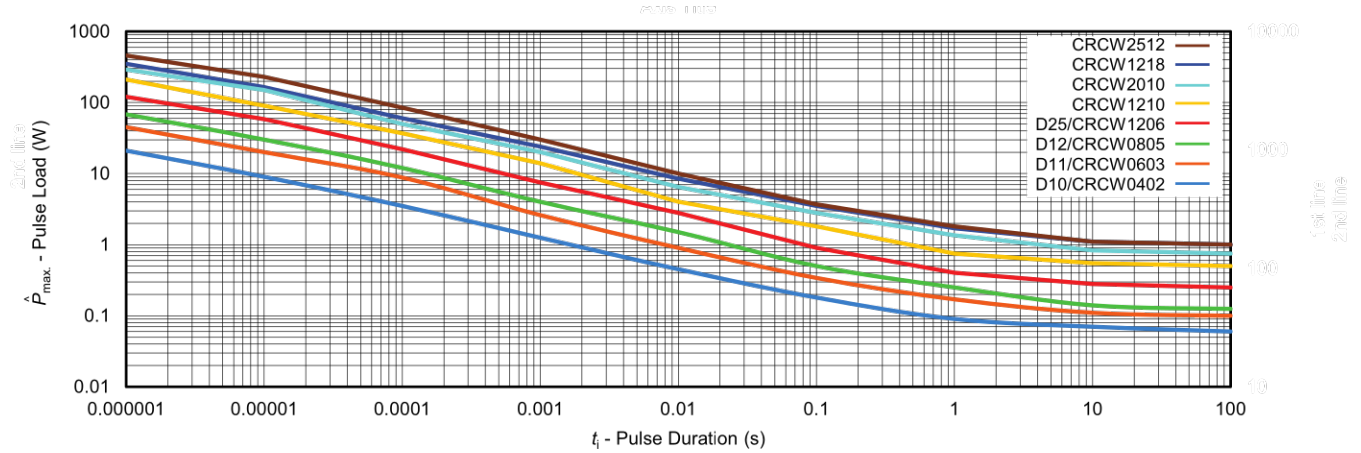
Maximum pulse load, single pulse; applicable if \bar{P} \rightarrow 0 and n < 1000 and \hat{U} = \hat{U}_{max} ; for permissible resistance change equivalent to 8000 h operation
