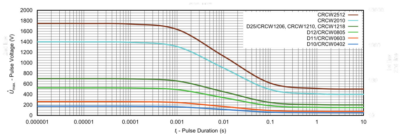
Maximum pulse voltage, single and continuous pulses; applicable if \hat{P} = \hat{P}_{max} ; for permissible resistance change equivalent to 8000 h operation
