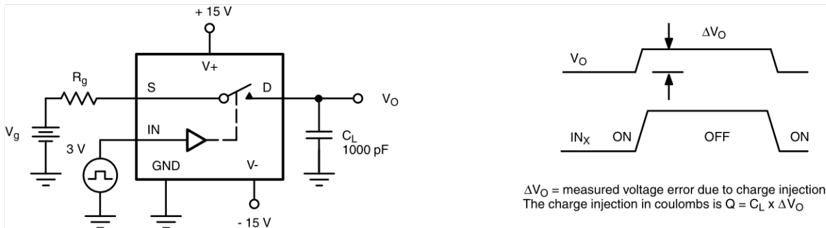
Figure 5. Charge Injection
