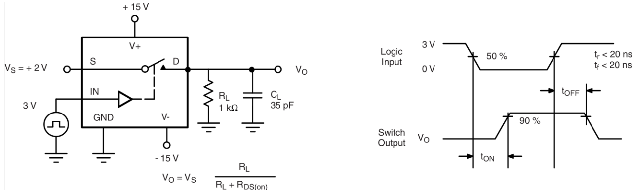
Figure 2. Switching Time
