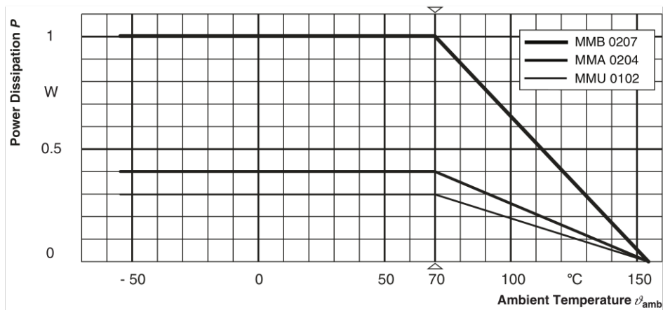
Derating - Power Operation Mode
