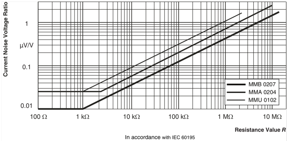
Current Noise Voltage Ratio
