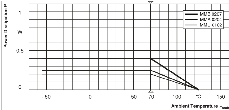
Derating - Standard Operation Mode
