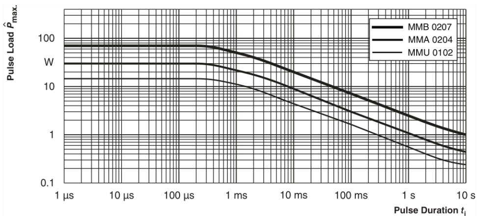
Single Pulse for R < 10 Ω
