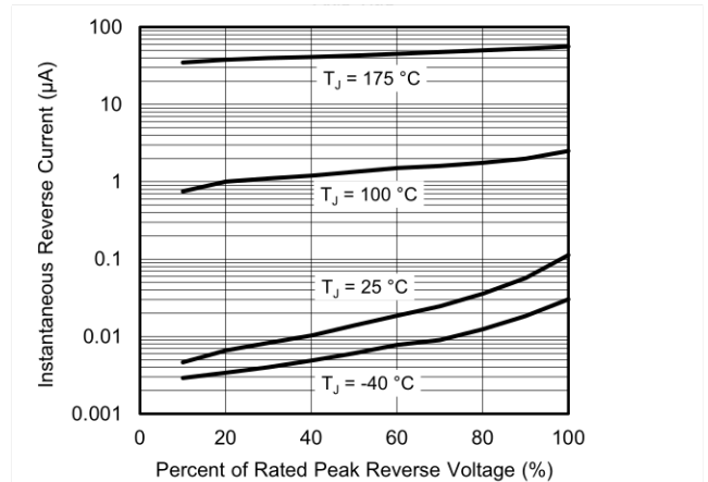
Fig. 4 - Typical Reverse Leakage Characteristics
