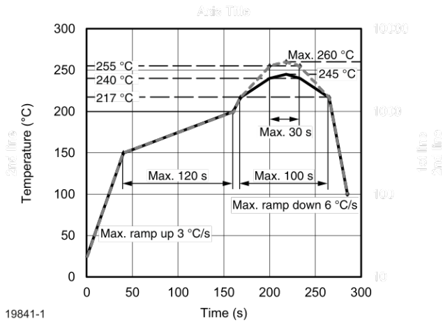
Fig. 21 - Lead (Pb)-free Reflow Solder Profile according to J-STD-020
