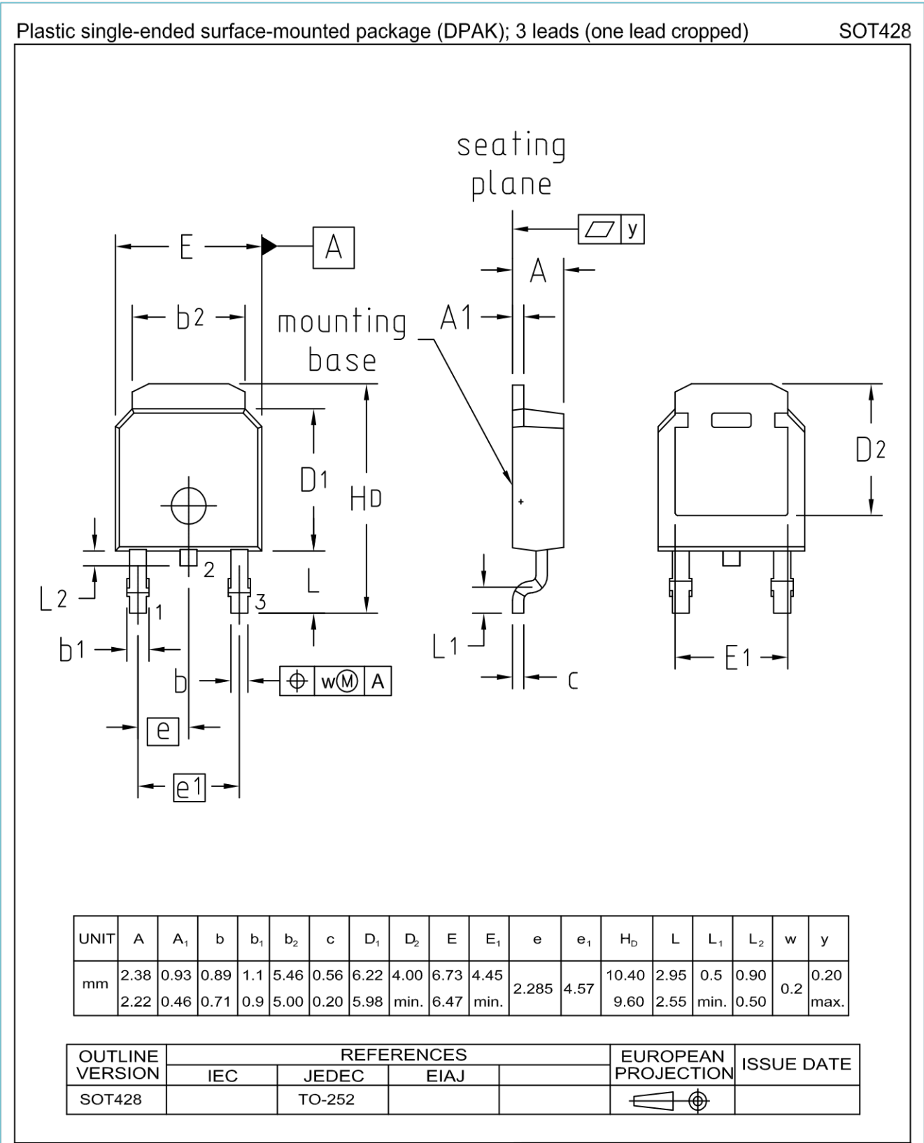
Fig. 12. Package outline DPAK (SOT428)
