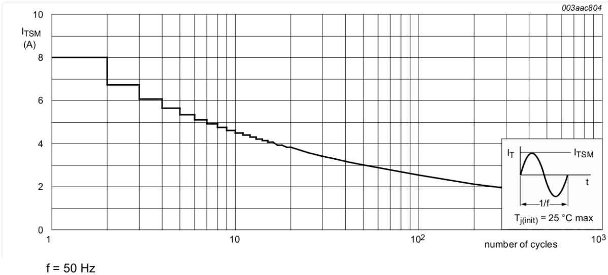
Fig. 3. Non-repetitive peak on-state current as a function of the number of sinusoidal current cycles; maximum values
