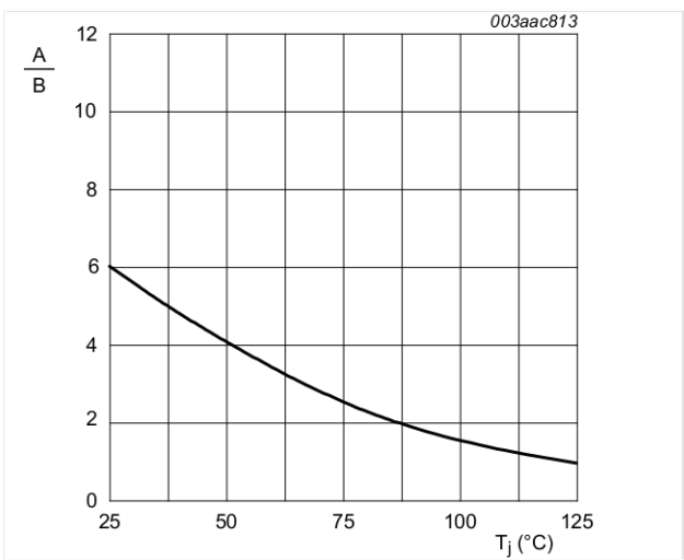
Fig. 11. Normalized rate of rise of off-state voltage as a function of junction temperature
