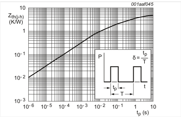
Fig. 3. Transient thermal impedance from junction to heatsink as a function of pulse width
