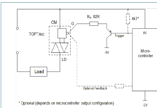
Fig. 16. DC triggering from 5 V microcontroller
