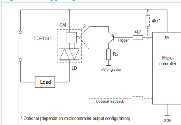
Fig. 18. DC triggering from 3.3 V microcontroller
